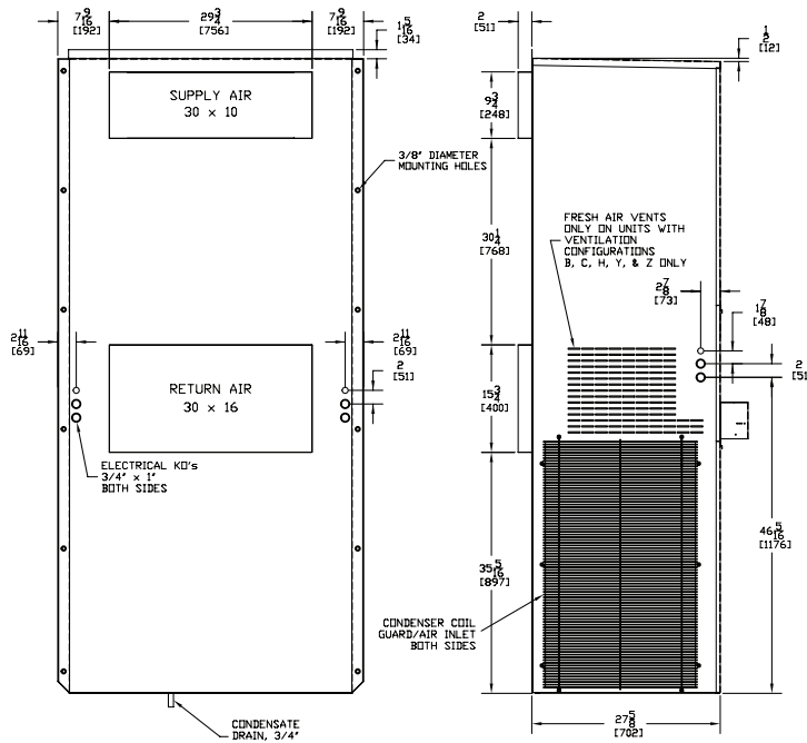
REAR VIEW
